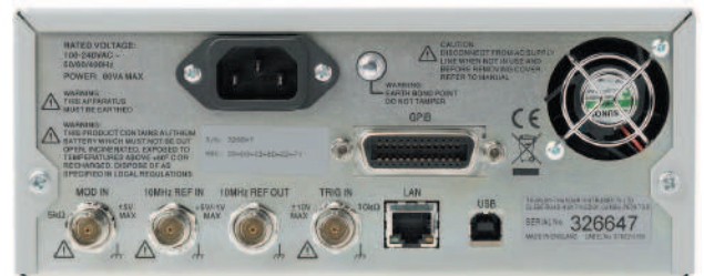
Rear panel mounts the digital interfaces and the rear I/O connectors. (Note: GPIB interface is an option)
